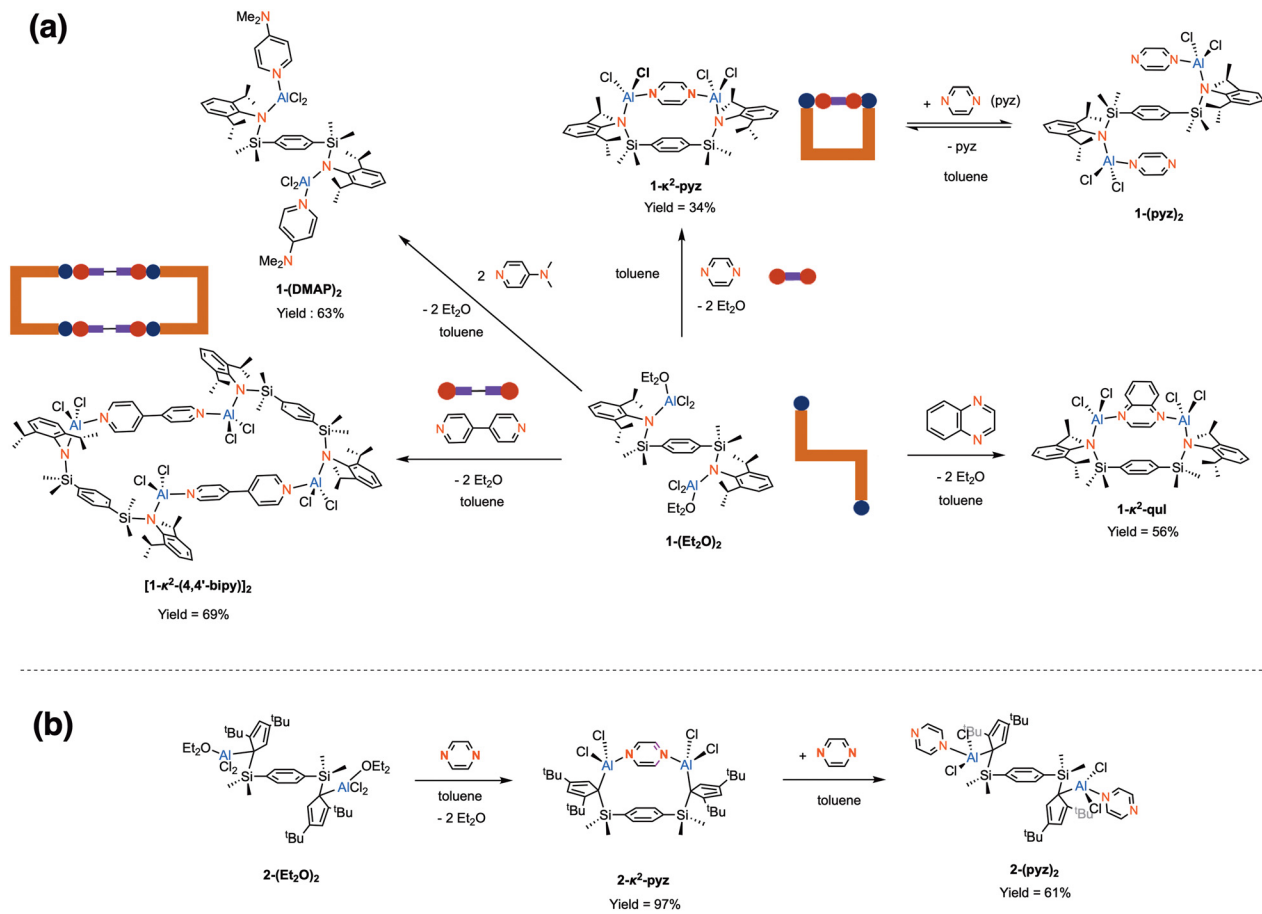
Scheme 2 Reactivity of (a) 1-(Et 2 O) 2 and (b) 2-(Et 2 O) 2 .
