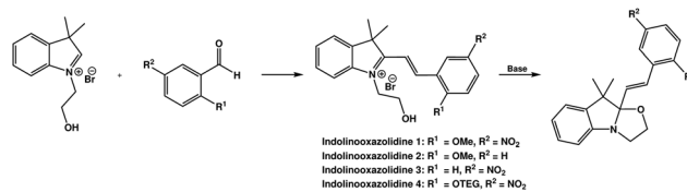
Fig. 2 The synthesis of indolinooxazolidines. A functionalized aromatic aldehyde is condensed with an indolium bromide salt, which gives a salt of the ring-opened indolinooxazolidine. The salt is then ring-closed using an inorganic base to provide the final photoswitch. Here, triethylene glycol ethyl ether is shortened to TEG.
