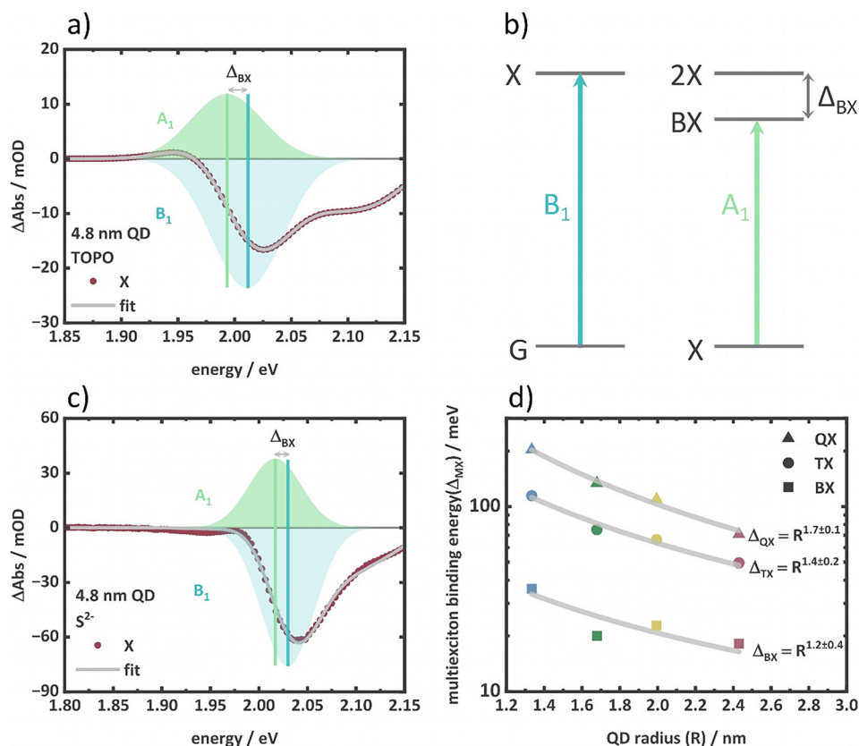
Fig. 5 The \text{A}_1 and \text{B}_1 peaks obtained from the multi-Gaussian fitting of the X spectra with eqn (S3) (ESI†) of 4.8 nm (a) TOPO-capped and (c) \text{S}^{2-} -capped QDs. The figures demonstrate the extent of the \text{A}_1 and \text{B}_1 overlap, which determines the \Delta_{\text{BX}} . (b) Excitonic state diagram representing the optical transitions corresponding to \text{A}_1 and \text{B}_1 in the X species. (d) Radius dependency ( \Delta_{\text{MX}} \propto R^n ) of \Delta_{\text{MX}} of BX, TX and QX obtained from the multi-Gaussian fitting of eqn (S3)–(S6) (ESI†).
