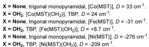
Fig. 17 Schematic representation of complexes 19 and 19' (left); CASSCF-computed principal magnetic anisotropy axes ( D_{xx} , D_{yy} , and D_{zz} ) are shown as pink dotted lines for the cobalt complex (a, 19a and b, 19a' ). The blue arrow highlights the direction and orientation of the D_{zz} , while the green arrows represent the molecular orientation axes (right), 94 adapted/reproduced from ref. 94 with permission from The Royal Society of Chemistry, 94 copyright 2018.
