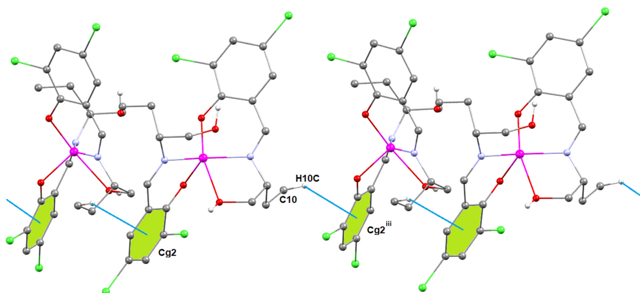
Fig. 5 C–H \cdots π interactions of complex 2A. Only the relevant hydrogen atoms are shown for clarity.
