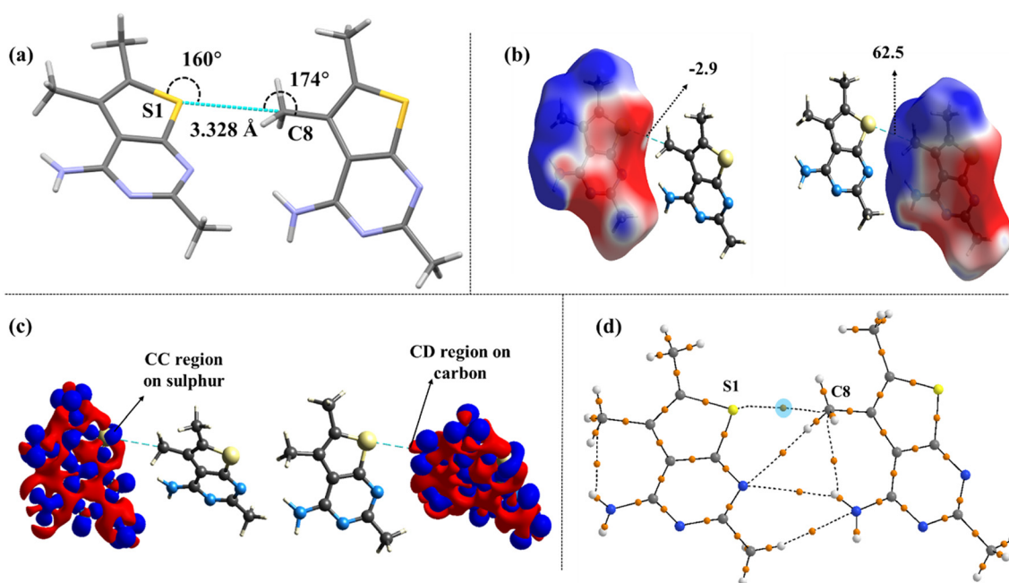
Fig. 14 (a) Distance and directionality of S \cdots C ( \sigma hole) tetrel interactions in compound 2 ; (b) MESP mapped over the Hirshfeld surface (values in \text{kJ mol}^{-1} ); (c) deformation density plot depicting the CC and CD regions; (d) QTAIM analysis validates the existence of bond critical points (highlighted in blue circles) in dimeric motifs.
