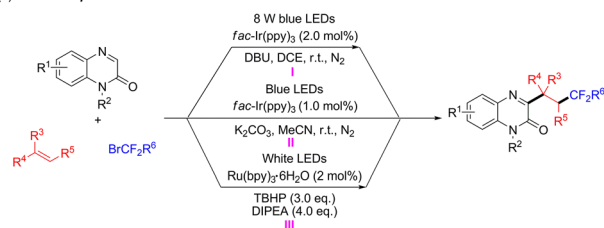
(b) Visible-light-promoted difluoromethyl radical formation via EDA complex
