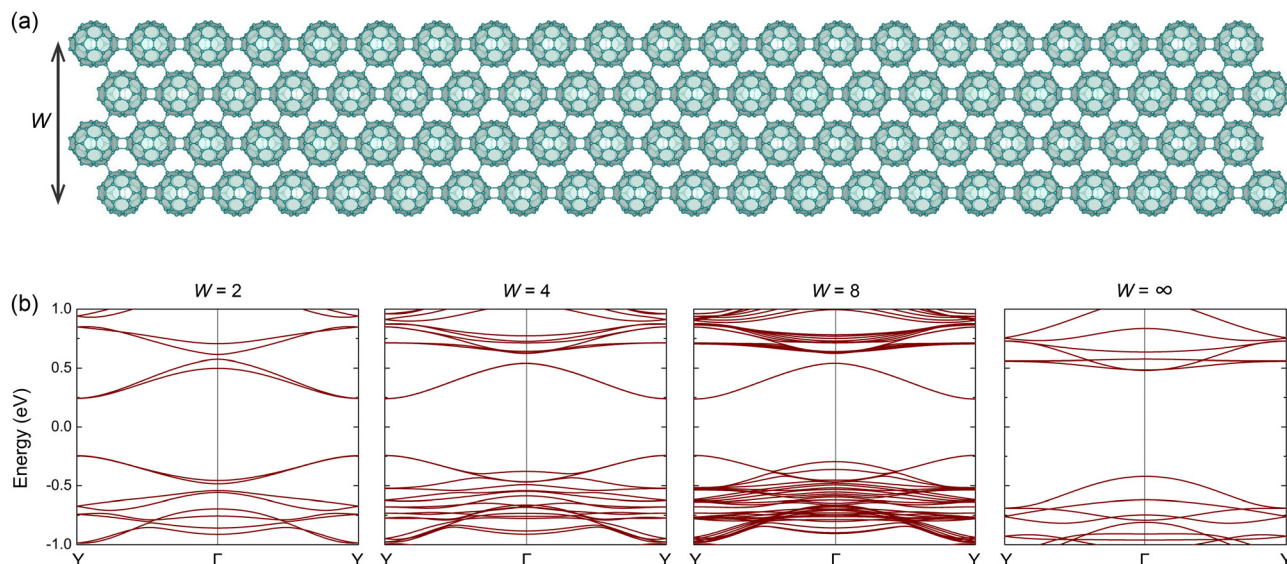
Fig. 16 (a) Crystal structures of a representative qHP-AC nanoribbon, and (b) their corresponding band structures as a function of W . 221
