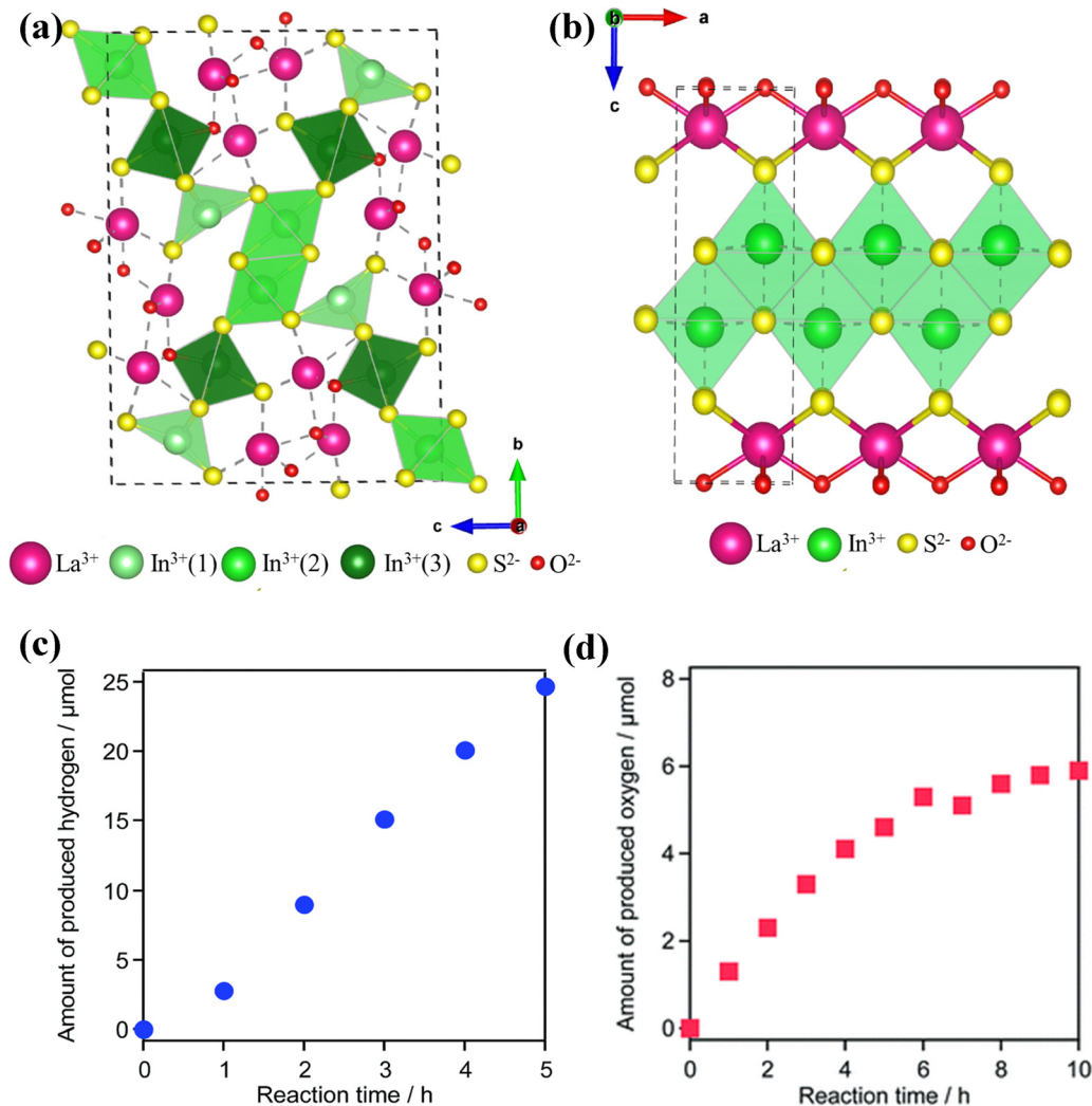
Fig. 5 Structural representation of \text{LaOInS}_2 material with (a) alpha model of Pbcm symmetry and (b) metastable layered model of P21/m symmetry; below, the water splitting properties of the metastable layered phase of \text{LaOInS}_2 are shown including (c) \text{H}_2(\text{g}) evolution for 0.75 wt% Pt/LaOInS 2 and (d) \text{O}_2(\text{g}) evolution for 0.5 wt% IrO 2 /LaOInS 2 . Reproduced from ref. 95 with permission from the Royal Society of Chemistry.
