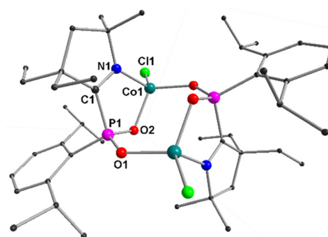
Fig. 2 Molecular structure of 4a . Hydrogen atoms are omitted for clarity. Co2 and O1 have 0.33 occupancy each. The ethyl group (C9 C10) is disordered with a site occupancy ratio of 53:47. Important bond lengths [Å], and bond angles [°]: Co1–Cl1 2.2034(11) [2.204], Co1–O1 1.941(2) [1.933], Co1–N1 2.042(3) [1.912], P1–O2 1.512(3) [1.554], P1–O1 1.514(3) [1.539], P1–C1 1.843(4) [1.824], N1–C1 1.282(5) [1.296]; O2–P1–O1 113.39(15) [114.96], P1–O2–Co1 115.66(15) [116.31].
