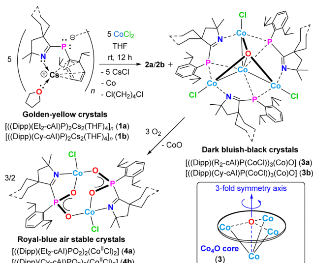
Scheme 1 Syntheses of Co 4 O clusters 3a–3b [Co1–Co2 2.7046(4)], and their reactivity with O 2 affording dimeric Co 2 O complexes 4a–4b . 2a–2b are the respective bis-(Dipp)(imino)-phosphene by-products, isolated separately as white needles (see ESI†).
