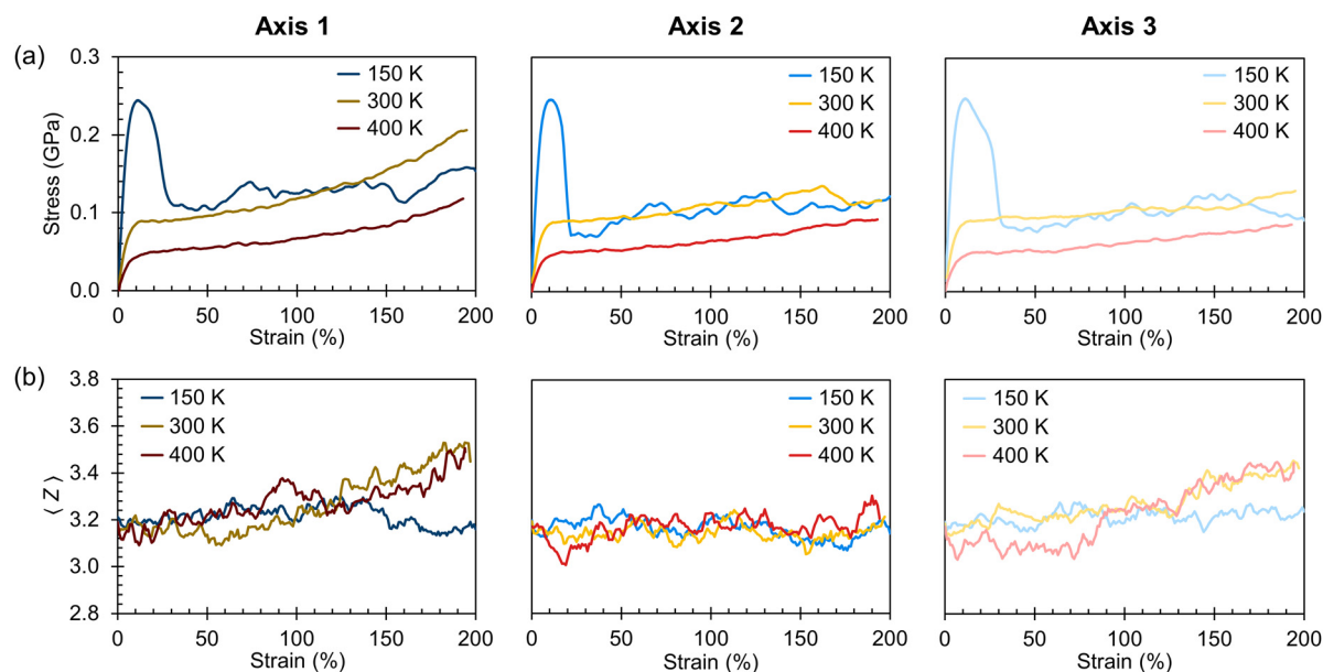
Fig. 5 (a) Stress–strain curves shown in Fig. 3(a) grouped instead by deformation axis and with a moving average of width 1.5 ns applied. (b) Average number of entanglements per chain, \langle Z \rangle , as a function of strain for each of the stress–strain curves in (a), also with a moving average of 1.5 ns applied.
