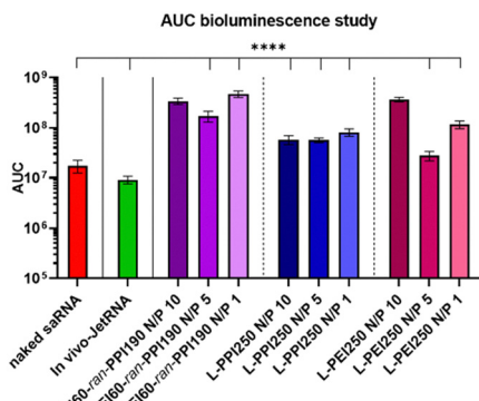
Fig. 8 Area Under Curve (AUC) in vivo bioluminescence. Data was obtained with the IVIS Lumina III (Total Flux [p/s]). * indicates significance of p \leq 0.05 , ** indicates significance of p \leq 0.01 , *** indicates significance of p \leq 0.001 , **** indicates significance of p \leq 0.0001 . All means were compared to each other with one-way ANOVA after testing for normality. Adjustment for multiple comparisons was performed using Tukey's multiple comparisons test in GraphPad Prism 8.4.3.
