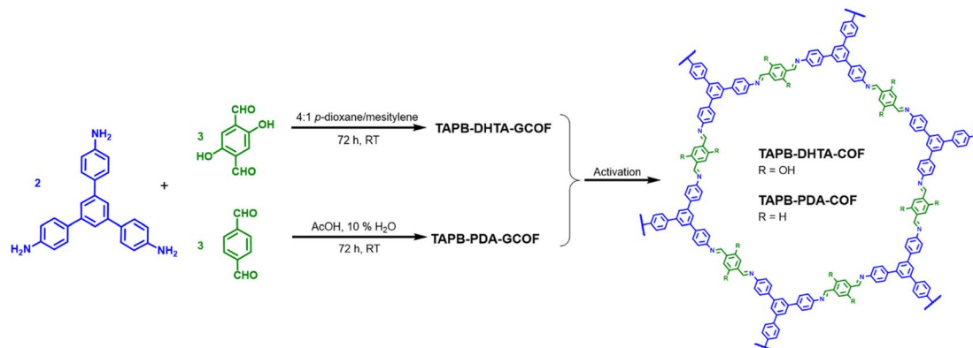
Scheme 1 Scheme of the synthetic procedure for TAPB-PDA-COF and TAPB-DHTA-COF in the form of gels and xerogels.
