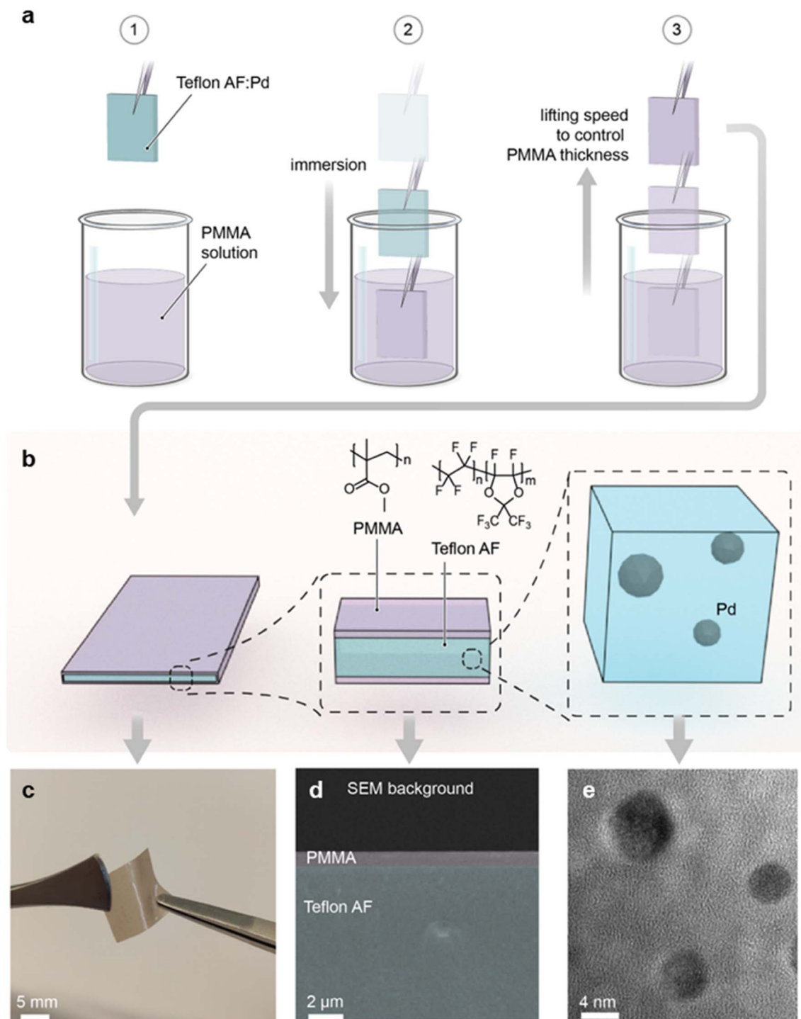
Fig. 2 Preparation and characterization of Teflon AF:PMMA core:shell structures. (a) Schematic of the dip coating process. (b) Architecture of Teflon AF:PMMA films coated with PMMA, including the chemical structures of PMMA and Teflon AF. (c) Photograph of a Teflon AF:PMMA film coated with PMMA. (d) False-colored SEM images of the cross section of a Teflon AF:PMMA film dip coated with PMMA at 5 mm s -1 . (e) TEM image of Pd nanoparticles in Teflon AF.
