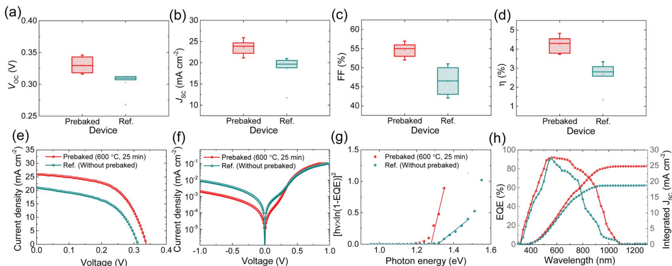
Fig. 3 Box plot of the PV parameters of the devices fabricated using the ref. (W.B.) SnS and prebaked "SnS + S" source films: (a) open circuit voltage ( V_{OC} ), (b) short circuit density ( J_{SC} ), (c) fill factor (FF), and (d) \eta , and (e) light J - V curve, (f) dark J - V curve, (g) bandgap extracted from the EQE profile, and (h) EQE response and integrated J_{SC} from EQE.
