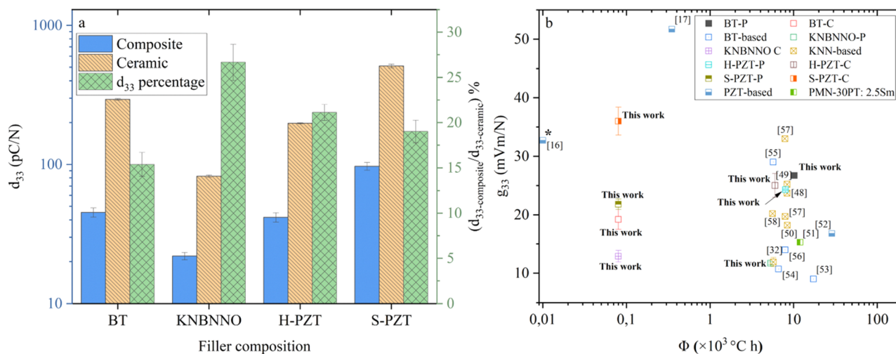
Fig. 5 (a) d_{33} of poled BT, KNBNNO, H-PZT and S-PZT ceramic and composite samples and ratio of the composite d_{33} value ( d_{33-composite} ) to the corresponding ceramic d_{33} value ( d_{33-ceramic} ) shown as a percentage ( (d_{33-composite}/d_{33-ceramic})\% ); and (b) dependence of longitudinal piezoelectric voltage coefficient ( g_{33} ) on the energy budget of fabrication ( \Phi ) for the ceramic and composite samples studied in this work as well as for selected high-performance counterparts reported in the literature. 16,17,32,48–58 In (b), the datapoint marked with * has an actual value of zero.
