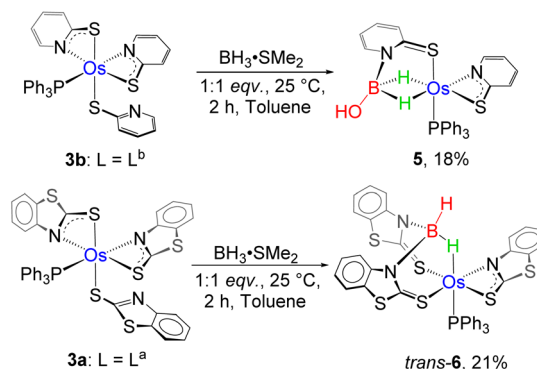
Scheme 3 B–H activation by paramagnetic Os(III)- N,S -chelated species, 3a–b .
