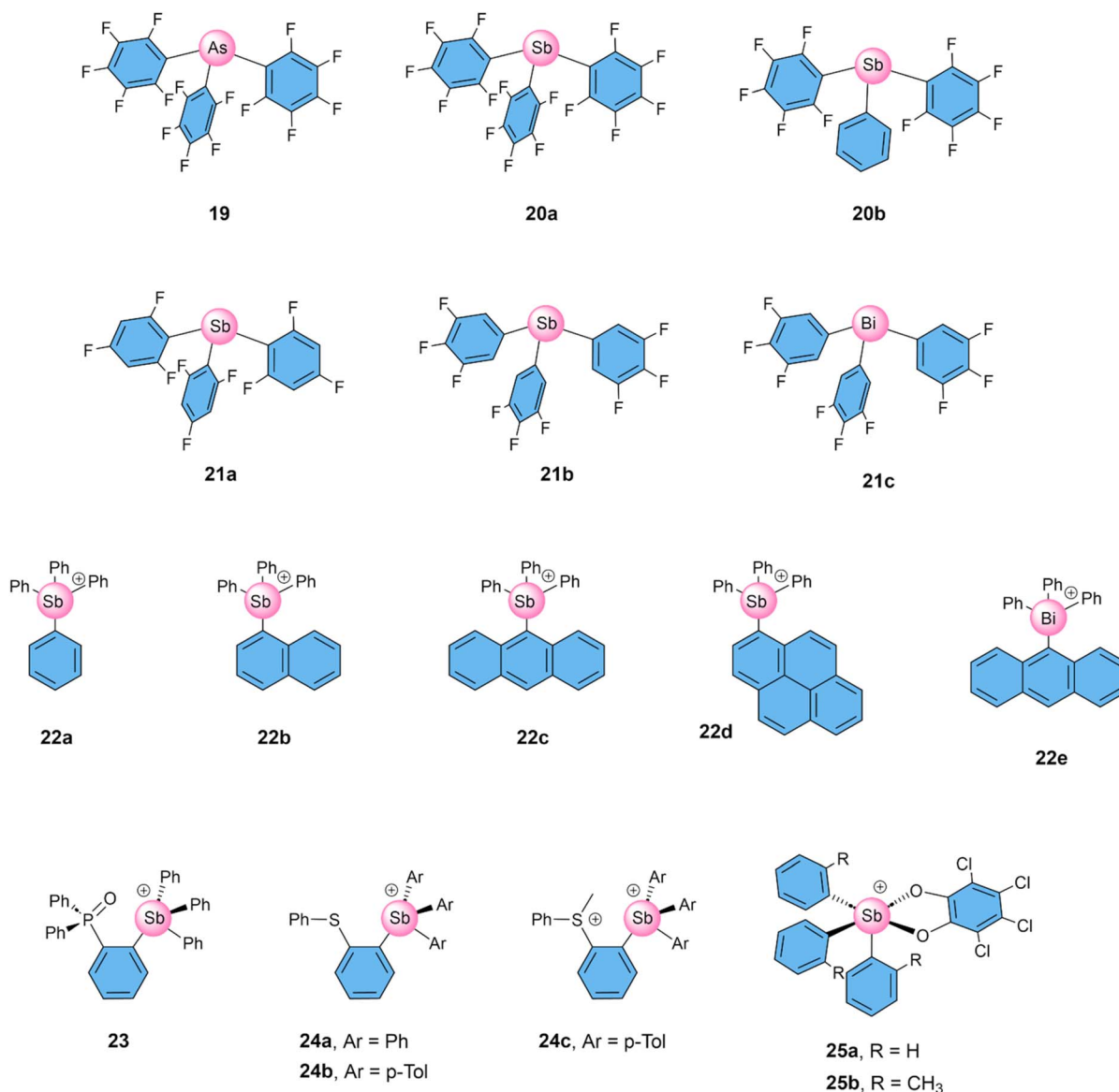
Fig. 8 Overview of compounds with PnB donors that have been studied as anion transporters.
