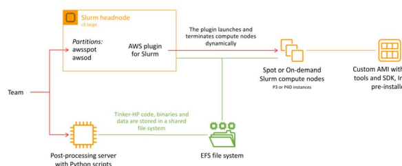
Fig. 2 Schematic representation of the cloud-based virtual cluster used for this study, enabling the use of AWS Spot and AWS On-demand (on demand) partitions and leveraging a shared elastic file system.
