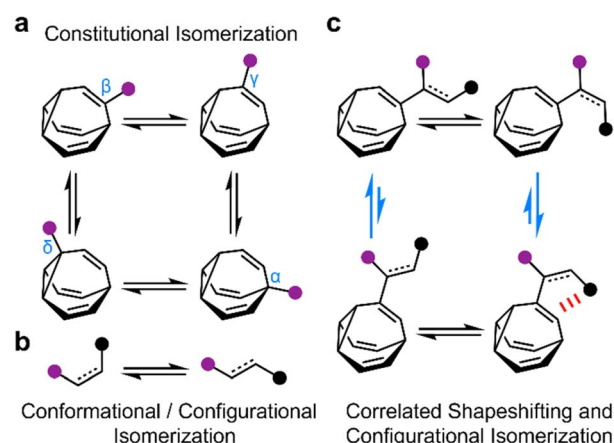
Fig. 1 The combination of (a) bullvalene shapeshifting rearrangements between constitutional isomers with (b) conformational and configurational changes by single bond rotations and E -to- Z isomerization are (c) correlated through noncovalent interactions (red) to bias the two bullvalene rearrangement equilibria in opposite directions (blue arrows). Black and purple circles represent appended functional groups.
