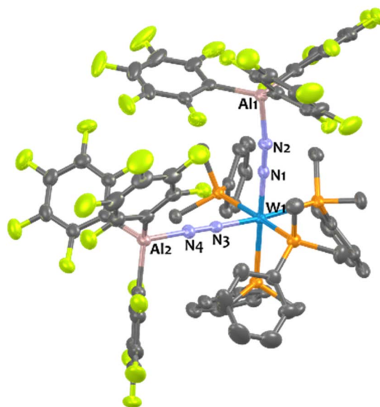
Fig. 8 Solid-state structure of 16 Al . Ellipsoids are represented with 30% probability. Hydrogen atoms have been omitted for clarity. Selected bond distances (Å) and angles (°): Al_1-N_2 1.915(3), Al_2-N_4 1.891(3), W_1-N_1 1.917(3), W_1-N_3 1.906(3), N_1-N_2 1.149(4), N_3-N_4 1.150(4), W_1-N_1-N_2 179.2(3), W_1-N_3-N_4 177.5(3), N_1-W_1-N_3 91.34(1), Al_1-N_2-N_1 168.5(3), Al_2-N_4-N_3 179.1(3).
