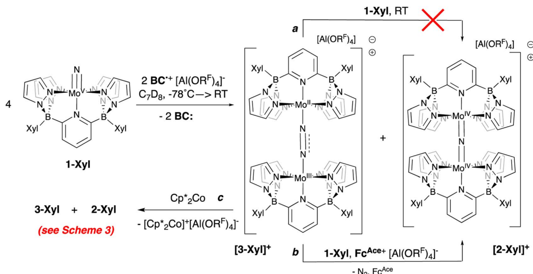
Scheme 5 Reaction of 1-Xyl with 0.5 equivalents of oxidant at -78^{\circ}\text{C} and subsequent transformations of the 1 : 1 mixture of [3\text{-Xyl}]^{+} : [2\text{-Xyl}]^{+} .
