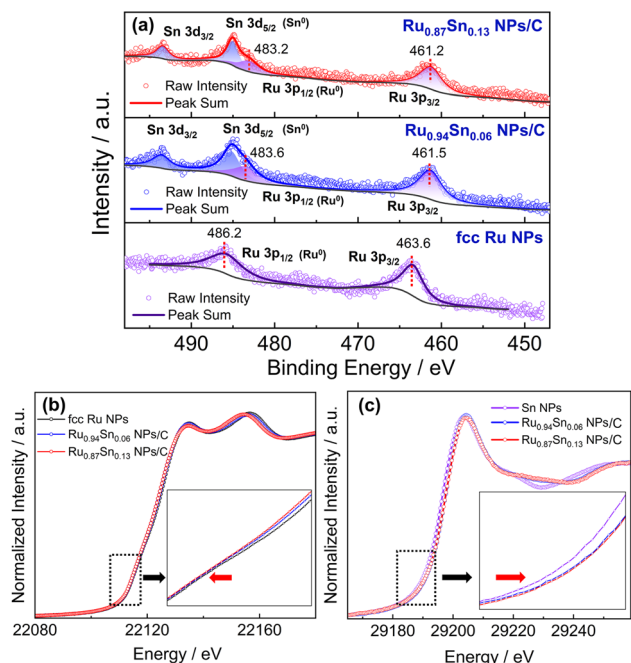
Fig. 5 (a) Ru 3p XPS spectra of fcc Ru NPs, Ru 0.94 Sn 0.06 NPs/C and Ru 0.87 Sn 0.13 NPs/C. The black curves serve as the background files. (b) Ru K-edge XANES spectra of fcc Ru NPs, Ru 0.94 Sn 0.06 NPs/C and Ru 0.87 Sn 0.13 NPs/C. (c) Sn K-edge XANES spectra of Sn NPs, Ru 0.94 Sn 0.06 NPs/C and Ru 0.87 Sn 0.13 NPs/C.
