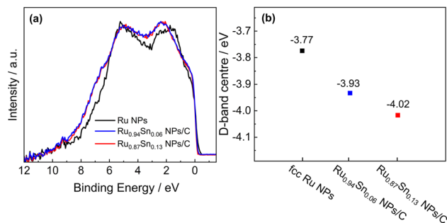
Fig. 4 (a) VB HAXPES spectra of Ru NPs, Ru 0.94 Sn 0.06 NPs/C and Ru 0.87 Sn 0.13 NPs/C. (b) d-band centres of Ru NPs, Ru 0.94 Sn 0.06 NPs/C and Ru 0.87 Sn 0.13 NPs/C.
