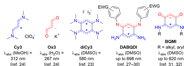
Fig. 1 Illustration of the coupling principle with trimethine derivatives (EWG = electron-withdrawing group).
