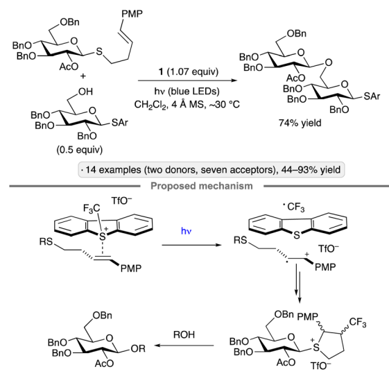
Scheme 3 O -Glycosylation via excitation of the EDA complex of a thioglycoside with Umemoto's reagent (1). PMP denotes 4-methoxyphenyl.
