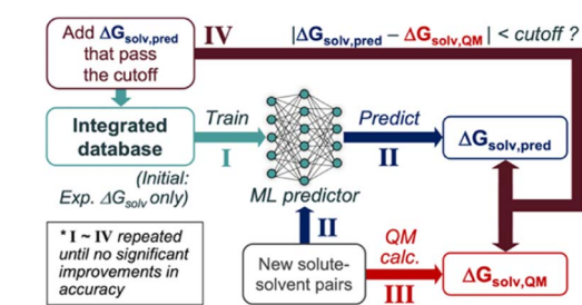
Scheme 1 The semi-supervised distillation (SSD) scheme for the predictive models of solubility.
