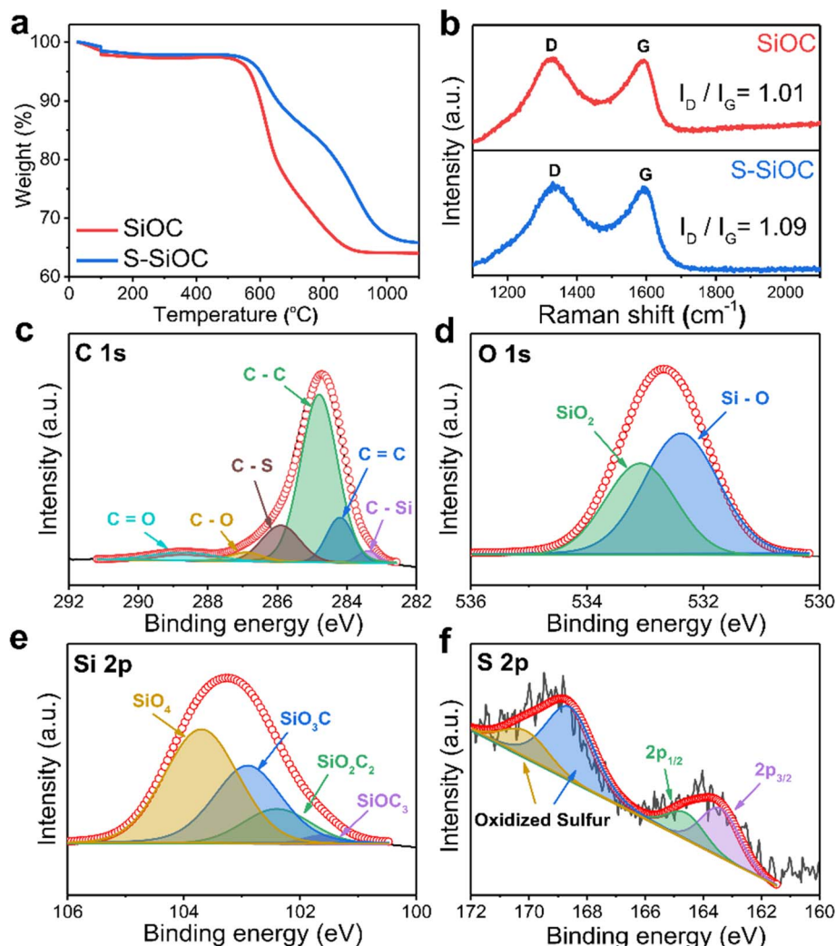
Fig. 2 (a) TGA curves of SiOC and S-SiOC at a heating rate of 5^\circ\text{C min}^{-1} under the air atmosphere. (b) Raman spectra of SiOC and S-SiOC. High resolution XPS spectra of (c) C 1s, (d) O 1s, (e) Si 2p, (f) S 2p in S-SiOC.
