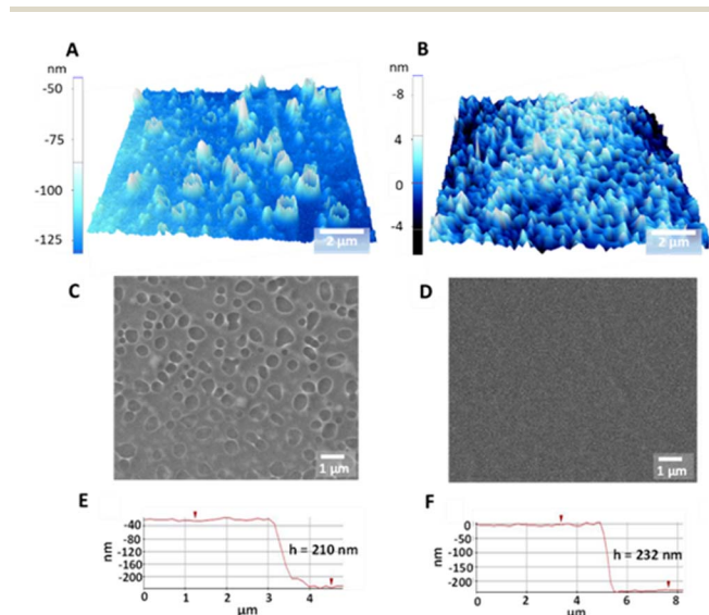
Fig. 3 3D AFM images of a nano rough (A) and a smooth (B) PEDOT:Tos/PDAC/PET film. SEM images of a nano rough (C) and a smooth (D) PEDOT:Tos/PDAC/PET films. AFM height profiles indicating the film thickness of a nano rough (E) and a smooth (F) PEDOT:Tos/PDAC/PET film.
