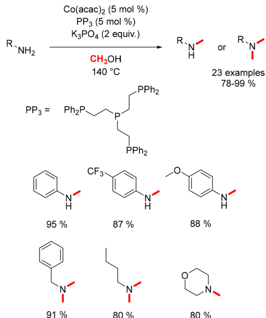
Scheme 39 Methylation of amines, as reported by Liu.
