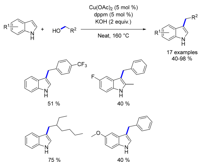
Scheme 105 C3-Alkylation of indoles.
