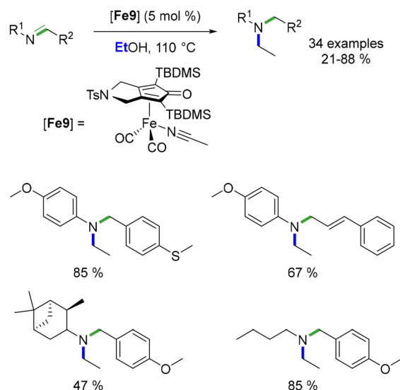
Scheme 28 Ethylation of imines, as reported by Bour.
