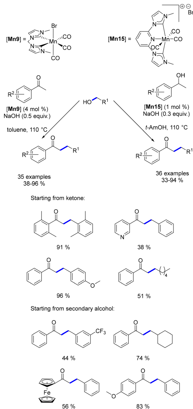
Scheme 72 Synthesis of \alpha -substituted ketones, as described by Ke.
