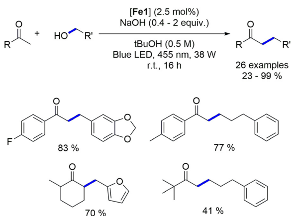
Scheme 110 Alkylation of aryl ketones with alcohols.
