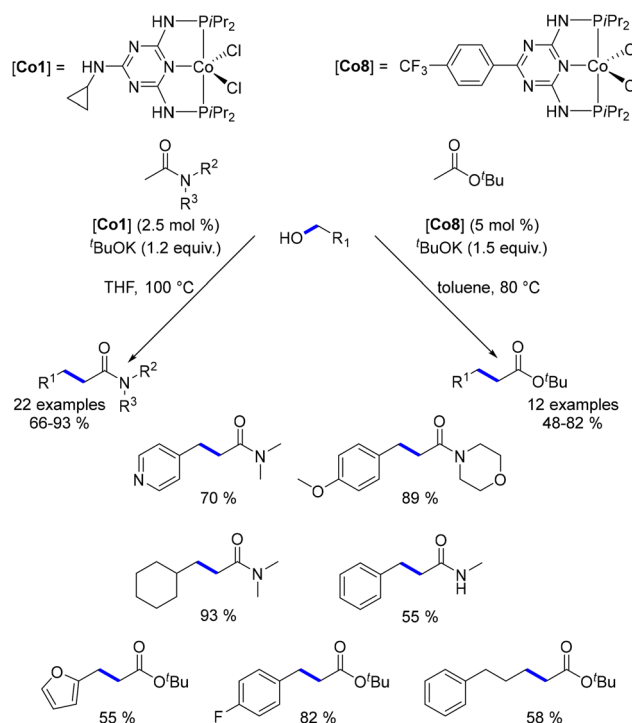
Scheme 91 C-Alkylation of amides and esters.
