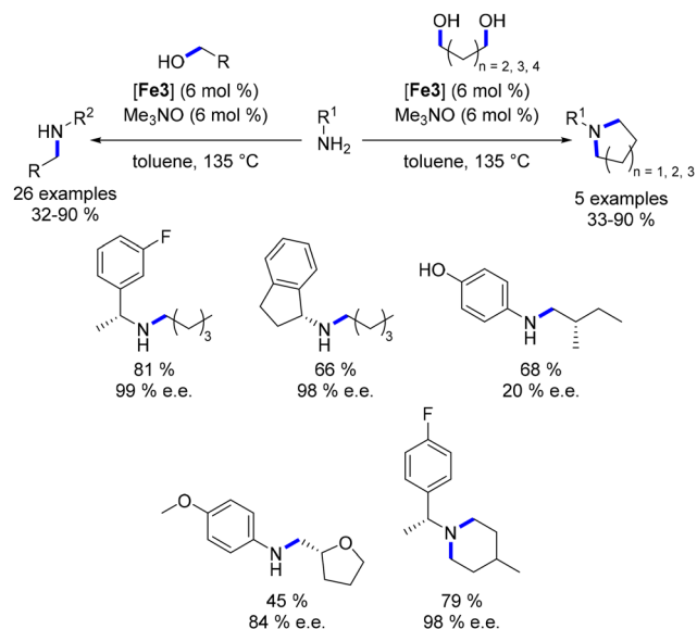
Scheme 23 Synthesis of chiral amines.
