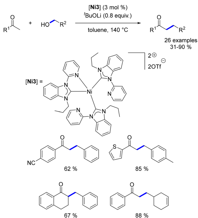
Scheme 104 Alkylation of ketones, as reported by Liu.
