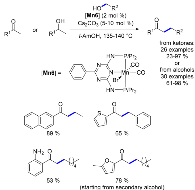
Scheme 65 Synthesis of α-substituted ketones.
