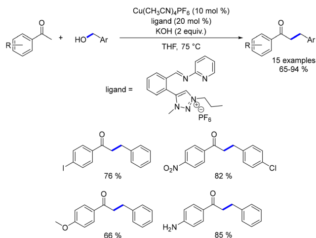
Scheme 106 Copper-catalysed alkylation of ketones.
