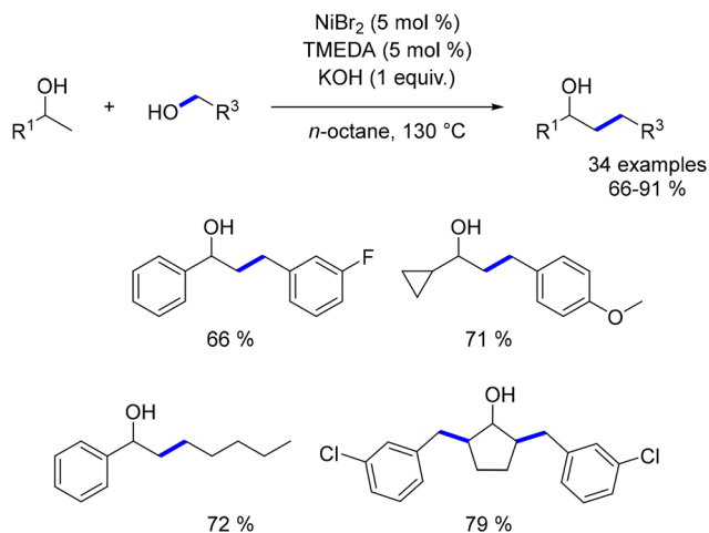
Scheme 103 Nickel-catalysed \beta -alkylation of alcohols.
