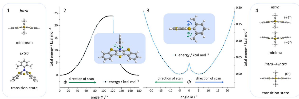
Fig. 3 Visualization of the relaxed geometry PES scans of N -inversion (2) and ring inversion (3) of N -aryls by the angle \phi of 3i (B3LYP/6-311G**, IEFCM CH 2 Cl 2 ). Most relevant minimum and transition state geometries of the relaxed geometry PES scan of N -inversion (1) and ring inversion (4) (B3LYP/6-311G**, IEFCM CH 2 Cl 2 ).
