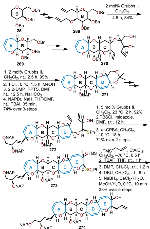
Scheme 43 Inoue, Hiram, and coworkers' synthesis of the A, D, and E oxepanes in CTX1B. 110,114,115
