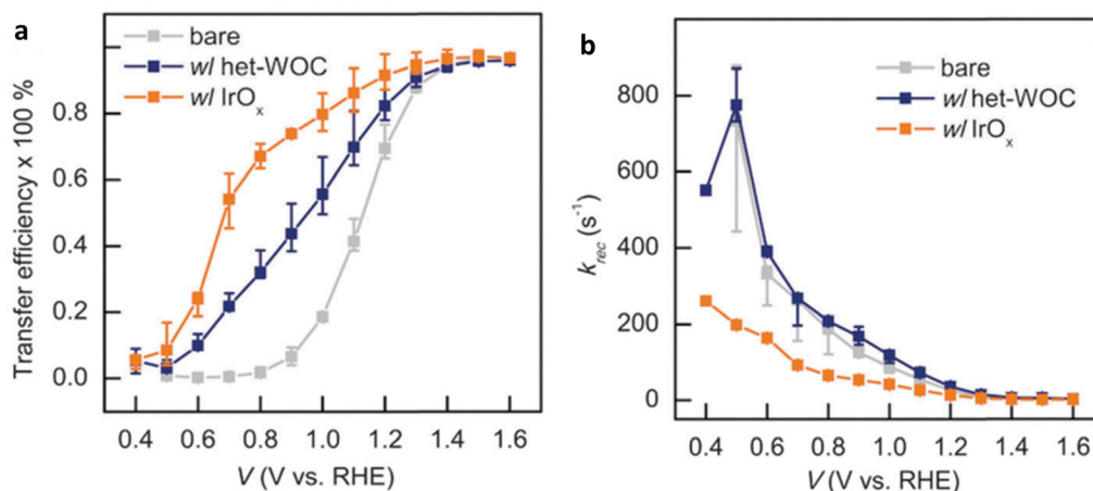
Fig. 19 Impact of heterogeneous catalysts (a). Transfer rate constant ( K_{trans} ) (b). Recombination rate constant ( K_{rec} ). Reproduced from ref. 152 with permission from Royal Society of Chemistry, copyright 2023.
