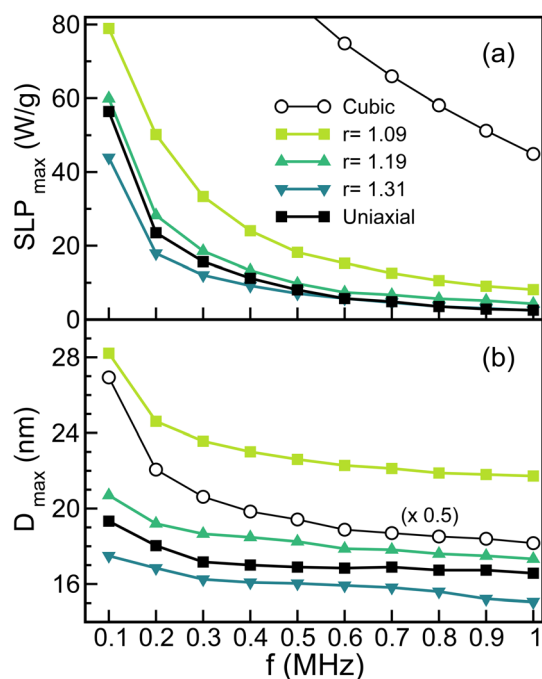
Fig. 8 Frequency dependence of the (a) maximum SLP and (b) the corresponding particle size extracted from the curves in Fig. 7 for different nanoparticle elongation ratios r = 1.09, 1.19 , and 1.31 (colored symbols) and also for the cases of only uniaxial (black squares) or only cubic contribution (empty circles) with K_{u,c} = 1.1 \times 10^4 \text{ J m}^{-3} . Notice that D_{\max} for the last case has been rescaled by 0.5.
