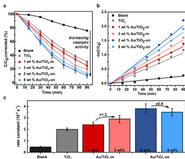
Fig. 4 Photocatalytic degradation of 15 \mu\text{M} MB under light illumination (200–2500 nm). (a) Fraction of MB concentration remaining in the reaction solution ( C/C_0 ) as a function of time. (b) MB decomposition kinetics expressed as -\ln(C/C_0) over reaction time, and (c) the correspondingly derived first-order rate constants.
