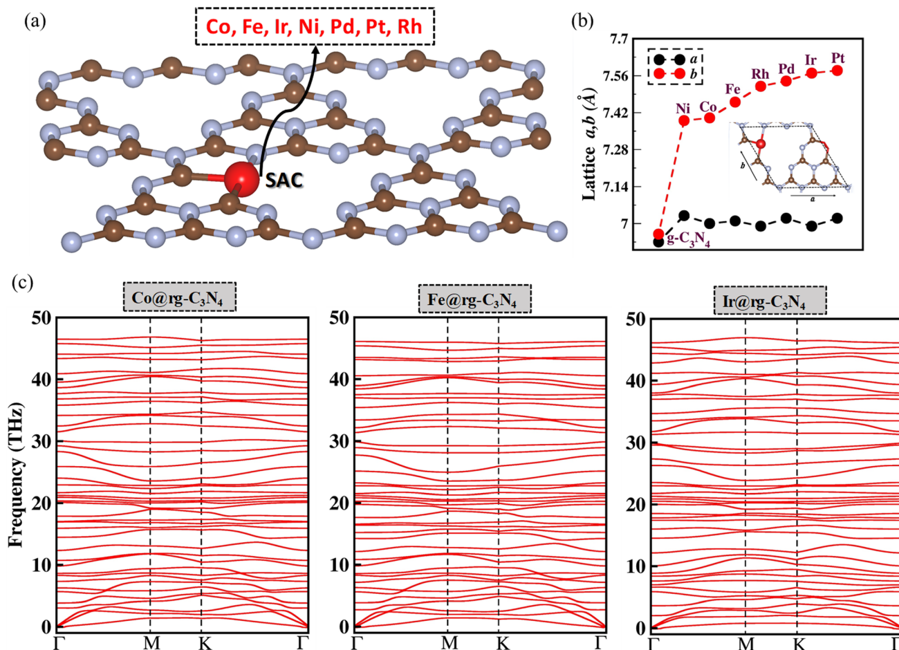
Fig. 1 (a) Perspective view of a SA adsorbed on the rg- \text{C}_3\text{N}_4 support. (b) Lattice constant of the SA@rg- \text{C}_3\text{N}_4 monolayer for a 1 \times 1 unit cell as represented in the inset. (c) Phonon spectra curves of SA@rg- \text{C}_3\text{N}_4 for SA = Co, Fe, Ir.
