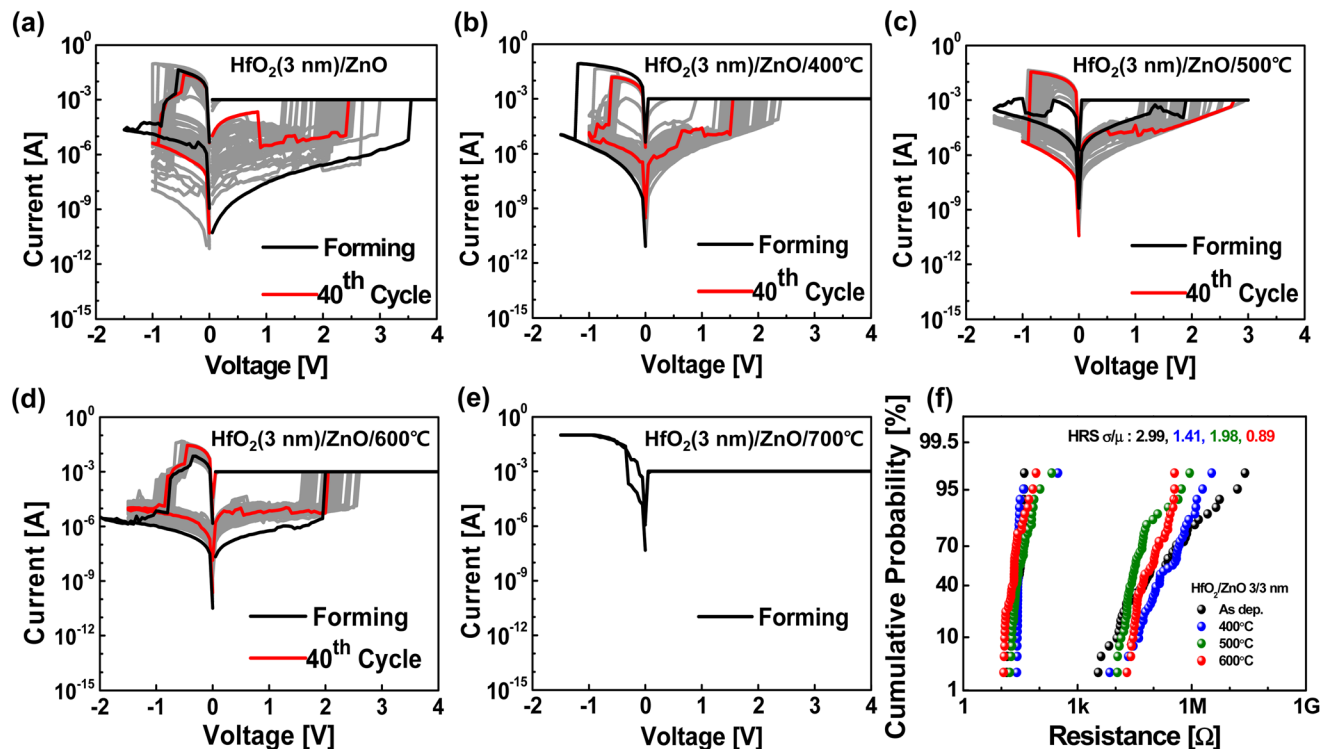
Fig. 5 Typical current–voltage ( I-V ) resistive switching behavior of bilayer \text{HfO}_2/\text{ZnO} synaptic devices (a) without and with thermal annealing at (b) 400 °C, (c) 500 °C, (d) 600 °C, and (e) 700 °C for 1 h in a \text{N}_2 ambient. (f) Distribution and cumulative probability of the high-resistance state (HRS) and low-resistance state (LRS) in 40 consecutive I-V sweeps for bilayer \text{HfO}_2/\text{ZnO} synaptic devices without and with thermal annealing, where the HRS and LRS were extracted at a read voltage of \pm 0.3 V.
