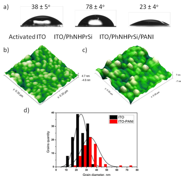
Fig. 1 Properties of the ITO/PhNHPPrSi/PANI surface: (a) the averaged water contact angles of the bare ITO, ITO/PhNHPPrSi, and ITO/PhNHPPrSi/PANI surfaces; (b) AFM image of the bare ITO and (c) the ITO/PhNHPPrSi/PANI surfaces; (d) the statistical distributions of grain diameters (the histograms are mean distributions of the grains diameters) on the surfaces.
