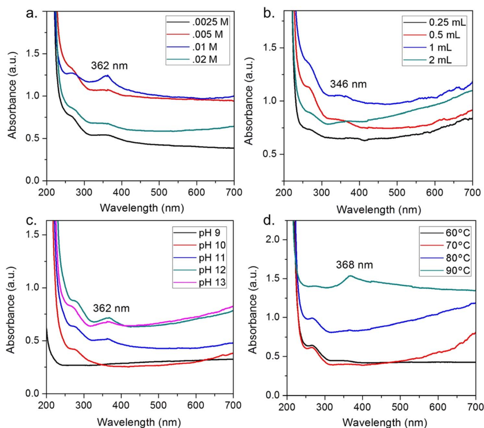
Fig. 6 Effect of factors on ZnO biosynthesis using Nyctanthes arbor-tristis floral extract, (a) concentration of \text{Zn}^{2+} , (b) volume of floral extract added into 50 mL of 0.01 M \text{Zn}^{2+} solution, (c) pH of the solution, (d) temperature of the solution. Reproduced with permission of Elsevier from ref. 59. Copyright 2018.
