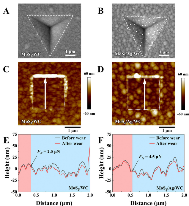
Fig. 3 Micro-mechanical properties of MoS 2 /WC and MoS 2 /Ag/WC nanomultilayer films. (A) and (B) SEM images of indentations from 50 mN nanoindentation tests performed on MoS 2 /WC and MoS 2 /Ag/WC nanomultilayer films. (C) and (D) SPM images showing topographical variations of worn surfaces after nano wear tests of MoS 2 /WC and MoS 2 /Ag/WC nanomultilayer films. Testing areas (2 × 2 μm 2 ) and directions marked by white dashed squares and arrows, respectively. (E) and (F) Corresponding 2D profiles along the white arrows marked in (C) and (D), respectively.
