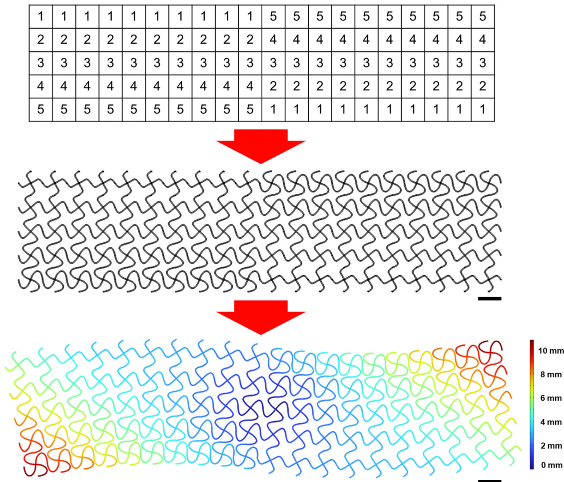
Fig. 11 Sine wave-shaped thermal deformation mode (all the scale bars are 40 mm).
