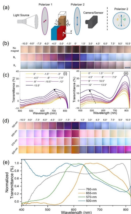
Fig. 4 (a) Schematic illustration of ORD measurement setup. (b) ORD images of \text{Ag@Fe}_3\text{O}_4 nanoparticle dispersion under no magnetic field or B_x and B_z fields. (c) The transmission spectra of the nanoparticle dispersion under B_x with varying negative (i) and positive (ii) \beta values. (d) ORD images of \text{Ag@Fe}_3\text{O}_4 nanoparticles with 760, 655, 570, and 500 nm extinction peaks under B_x with varying \beta values from -10.5 to 10.5^\circ . (e) The corresponding transmission spectra of the sample in (d) at \beta = 0^\circ . All the digital images in (b) and (d) share the same scale bar of 1 mm.
