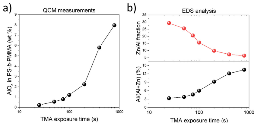
Fig. 2 (a) Variation of the \text{AlO}_x mass gain fraction of AZO infiltrated PS- b -PMMA with respect to the TMA exposure duration. (b) Plot of the atomic composition of Al and the atomic ratio of the Zn/Al in AZO nanostructures for different TMA exposure times. Here, the Al atomic composition within AZO is \text{Al at\%}/(\text{Al at\%} + \text{Zn at\%}) \times 100 , where respective atomic concentrations of Al and Zn were obtained from the EDS analysis that included Al, Zn, O, and Si ( i.e. , from the substrate) as the elements of interest (Table S1, ESI†).
