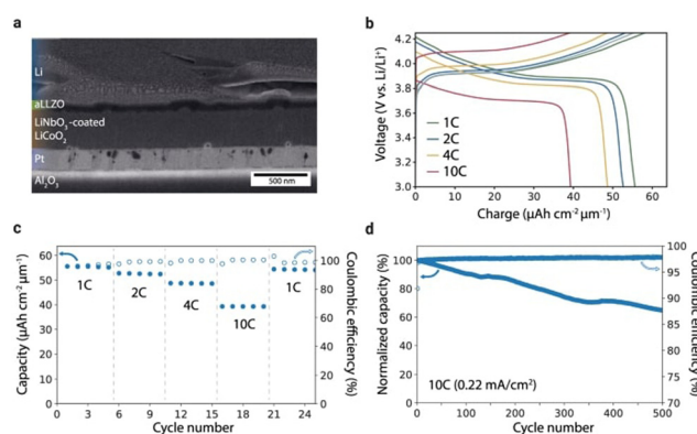
Fig. 13 (a) Cross-section SEM image of the battery stack. (b) Charge-discharge curves at different C rates (1C = 22 \mu\text{A cm}^{-2} ). (c) Discharge capacity and coulombic efficiency of the battery at different C rates. (d) Long-term cycling of the battery over 500 cycles at 10C (0.22 \text{mA cm}^{-2} ). 160 Copyright 2021 Springer Nature Limited.
