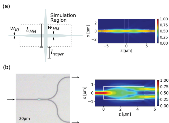
Fig. 2 (a) Schematic of the waveguide crossing device and (b) optical micrograph of an MMI-based 1 by 2 power splitter. The simulated top-down electric field profile ( |E_x|^2 ) for (a) and the electric field intensity profile ( |E_x|^2 ) for (b) are presented on the right. Reprinted with permission from ref. 46 © Optical Society of America.
