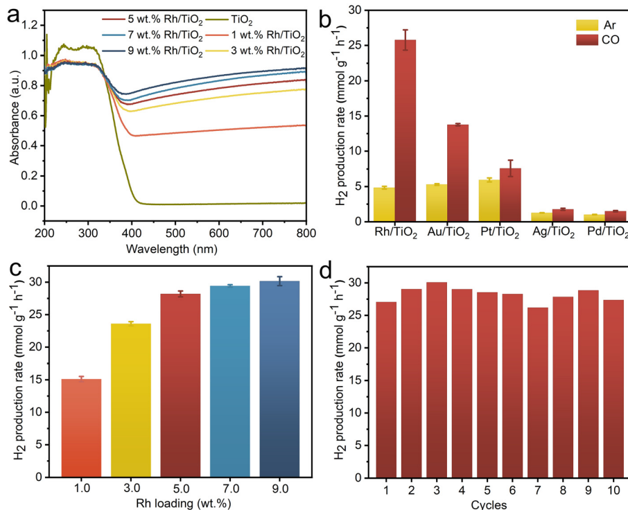
Fig. 3 (a) Absorption spectra for \text{TiO}_2 and x wt.% \text{Rh}/\text{TiO}_2 ; (b) triphase photocatalytic \text{H}_2 production rate for 5 wt.% \text{M}/\text{TiO}_2 ( \text{M} = \text{Rh}, \text{Au}, \text{Ag}, \text{Pt}, \text{Pd} ) in Ar or CO atmosphere; (c) photocatalytic \text{H}_2 production rate as a function of the loading amount of Rh in \text{Rh}/\text{TiO}_2 ; (d) cycling tests for \text{Rh}/\text{TiO}_2 . Reaction conditions: gas phase = 0.2 MPa of CO, liquid phase = 10 mL of \text{H}_2\text{O} , solid phase = 2 mg of photocatalyst immobilized on GDL (4 cm in diameter), light source = 365 nm LED ( 300 \text{ mW cm}^{-2} ). Error bars represent the standard deviation from at least three independent measurements.
