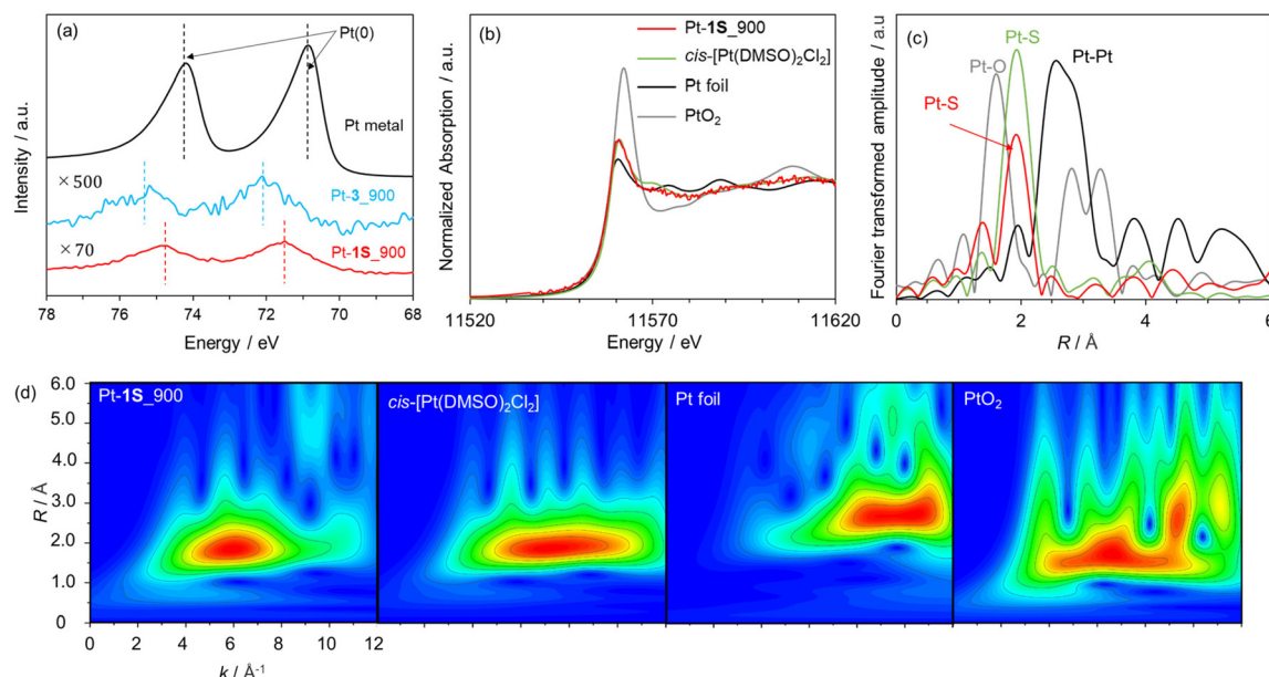
Fig. 5 (a) Pt 4f XPS spectra of Pt-1S_900, Pt-3_900, and Pt metal. (b) Pt L 3 -edge XANES spectra and (c) Fourier transforms of k 3 -weighted EXAFS oscillations for Pt-1S_900, cis -[Pt(DMSO) 2 Cl 2 ], Pt foil, and PtO 2 . (d) Wavelet transforms of Pt-1S_900, cis -[Pt(DMSO) 2 Cl 2 ], Pt foil, and PtO 2 .
