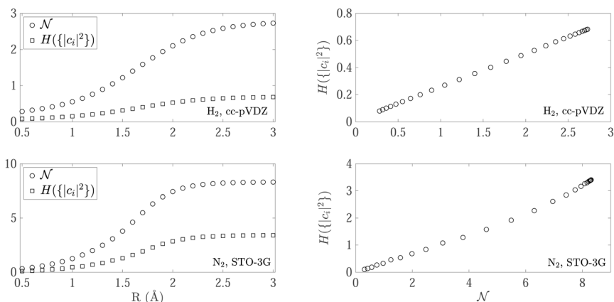
Fig. 7 Nonfreeness \mathcal{N} and Shannon entropy H(\{|c_i|^2\}) of the CI expansion coefficients in natural orbital basis for the full CI ground state of \text{N}_2 in the STO-3G basis at various internuclear distances R (left), and H(\{|c_i|^2\}) as a function of \mathcal{N} (right).
