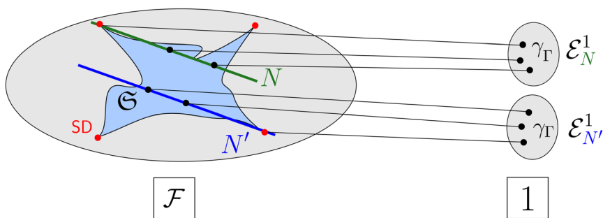
Fig. 3 Illustration of the one-to-one relation between the set \mathcal{G} (light blue) of free states on the Fock space \mathcal{F} (gray) and the sets of 1RDMs \mathcal{E}_N^1 for two different particle numbers N , N' . The red dots illustrate its extremal elements, which are the Slater determinants. For fixed particle number N , the free states \Gamma corresponding to 1RDMs \gamma_\Gamma \in \mathcal{E}_N^1 lie on a hyperplane with average particle number \langle \hat{N} \rangle_\Gamma = N .
