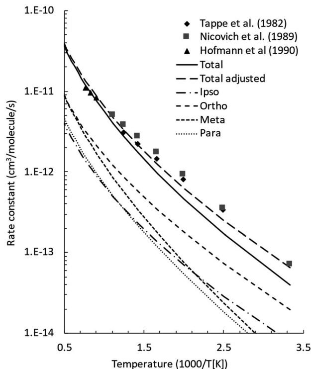
Fig. 6 Comparison between calculated (lines) and experimental (points) rate constants for \text{O}(^3\text{P}) addition to toluene. The total adjusted rate was determined by decreasing the energy barrier for all addition channels by 1.2 \text{ kJ mol}^{-1} , which is well within the uncertainty of the adopted theoretical model. Symbols: experimental rate constants from Tappe et al. , 24 Nicovich et al. , 23 and Hoffmann et al. 25
