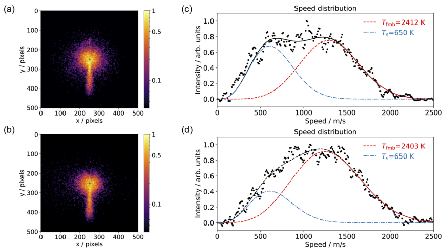
Fig. 4 Comparison of the velocity-map images of CO 2 from CO oxidation on Pd(110) at T_s = 650 \text{ K} and (a) a pure CO beam with p_{\text{O}_2} = 7.5 \times 10^{-8} \text{ mbar} ; (b) a 10% O 2 in He beam with p_{\text{CO}} = 5 \times 10^{-6} \text{ mbar} in the scattering chamber. The green dot in (a) and (b) represents the center of the image (zero velocity). (c) and (d) show the corresponding speed distributions (black dots) for CO 2 from (a) and (b), respectively. The speed distribution is fitted (black dashed) with one slow component (blue dashes) and one fast component (red dashes).
