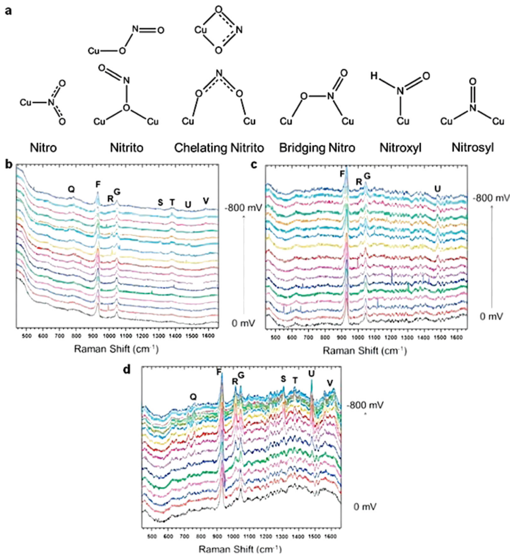
Fig. 15 (a) Adsorption modes of nitrite, nitric oxide, and HNO on the Cu surface. Electrochemical in situ SHINERS spectra collected from (b) Cu (100), (c) Cu (111), and (d) Cu (110) in a 0.1 M \text{HClO}_4 solution with 0.05 M \text{HNO}_3 and 10 mM HCl at a potential between 0 and -0.8 V vs. Ag/AgCl. Reprinted with permission from ref. 157 Copyright 2016 Elsevier Ltd.
